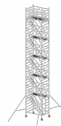
RS4S135x185x1000C
