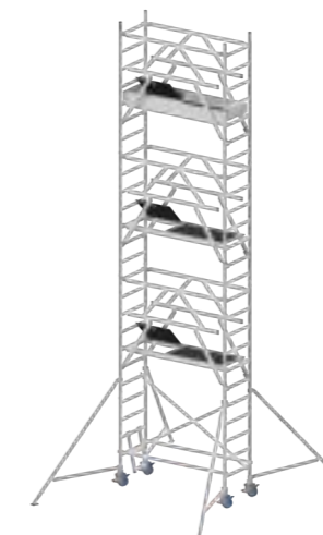
RS4S075x185x600
